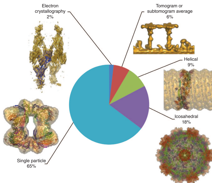
Figure 2 Holdings of the EMDb by 3DEM technique. A representative example of each category is shown: single particle, human \alpha B-crystallin 24-mer (EMD-1894, PDB 2YGD); icosahedral, cytoplasmic polyhedrosis virus (EMD-5256, PDB 3IZX); helical, GMPPCP-stabilized human dynamin 1 \Delta PRD polymer (EMD-1949, PDB 3ZYS); tomogram or subtomogram average, radial spokes from Chlamydomonas reinhardtii flagella (EMD-1941); 2D crystal, pig gastric H + ,K + -ATPase with bound Bef and SCH28080 (EMD-1831, PDB 2XZB) 24 .
