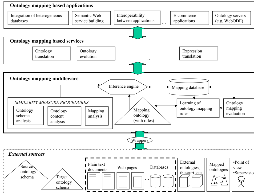
Fig. 1. Framework for automatic generation of ontology mappings
