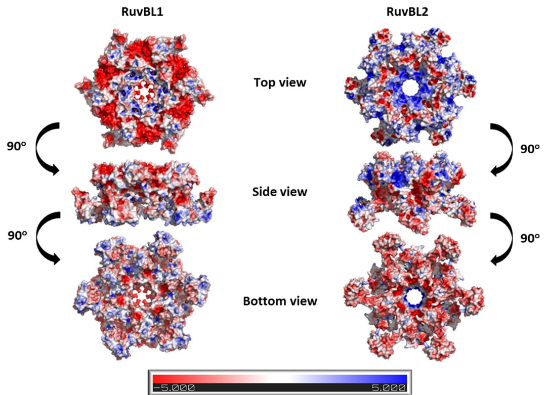
Figure 2. Surface charge distribution in the hsRuvBL1 and hsRuvBL2 hexamers. Differences in the distribution of amino acid residues at the surface of the rings may underlie their antagonistic activities. Colour by electrostatic potential on solvent accessible surface. Scale bar at the bottom, in kT/e.
