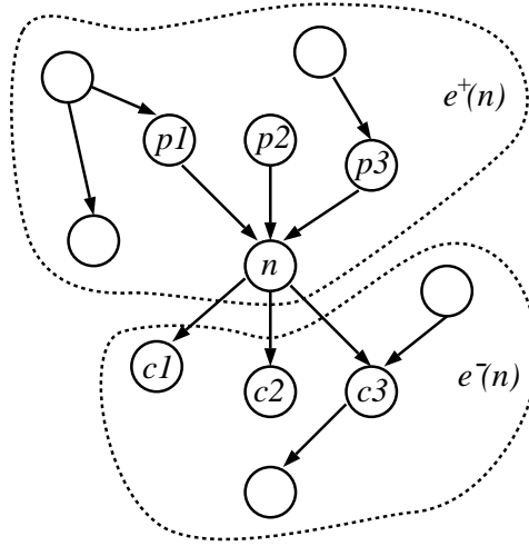
Fig. 3. Separation of evidence in singly connected graphs.
