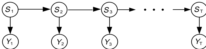
Fig. 1. A Bayesian network specifying conditional independence relations for a hidden Markov model.
