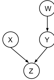
Fig. 2. A directed acyclic graph (DAG) consistent with the conditional independence relations in P(W, X, Y, Z) .
