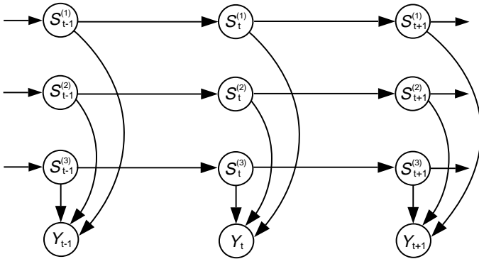
Fig. 5. A Bayesian network representing the conditional independence relations in a factorial HMM with M = 3 underlying Markov chains. (We only show here a portion of the Bayesian network around time slice t .)
